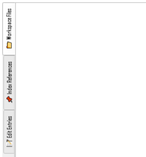
Figure 6. Views sidebar.
